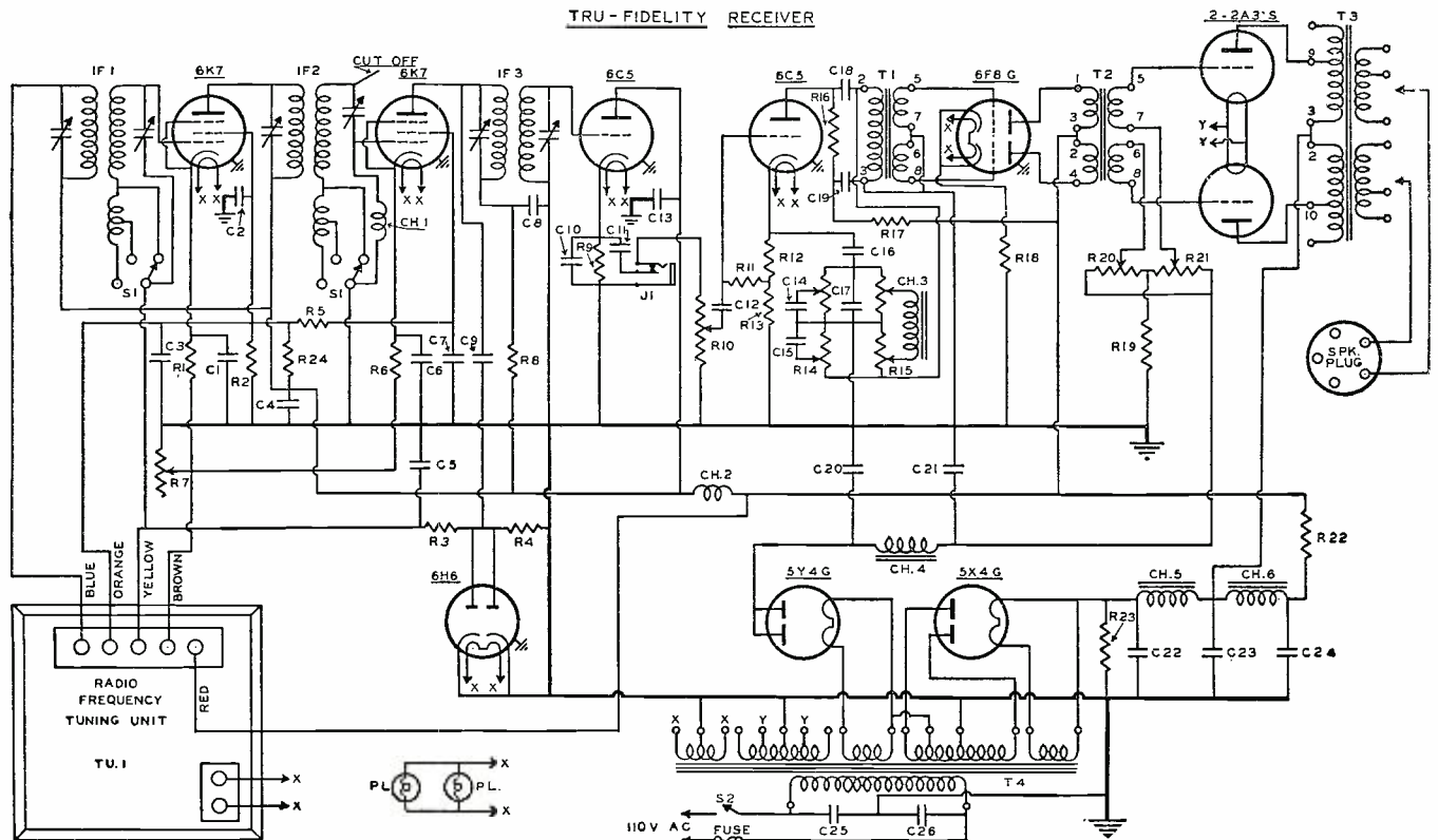
Circuit diagram of the True-Fidelity Receiver.
