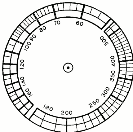
Dial layout detail.
