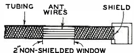
The assembled loop.
