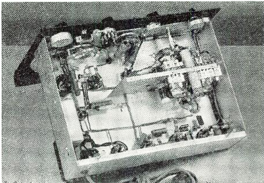
The cleanliness of the layout and the wiring materially help not only in the construction, but add to the efficiency of the unit as well.
