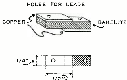
DETAIL 2 MMF. CONDENSER Condenser construction details.
