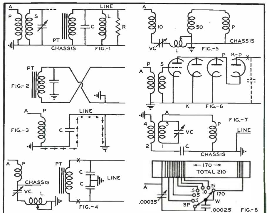
Various interference circuits described by the author.
