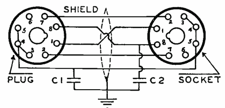
EXTENSION FOR 6J7 TUBE
