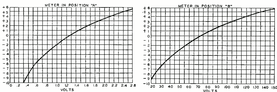
Conversion charts for converting DB meter readings to volts.
