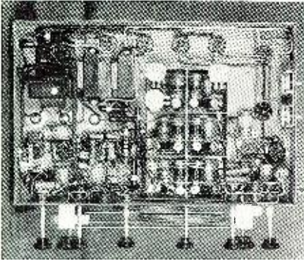
Underchassis view of the receiver. Note coil position and wiring.
