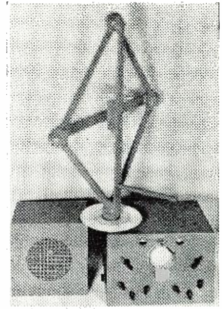
The receiver described by the author.
