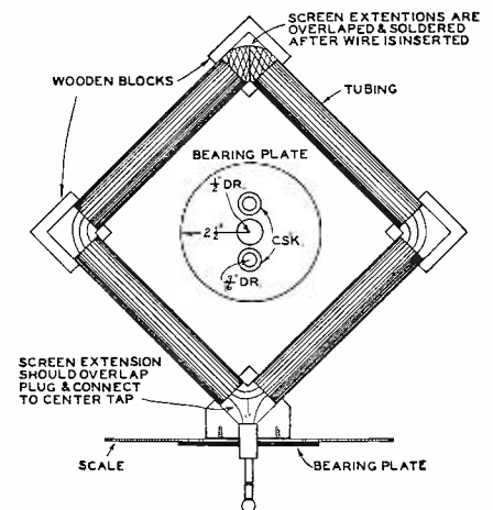
The assembled loop.
