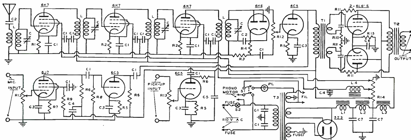
Circuit diagram of the superhet receiver.
